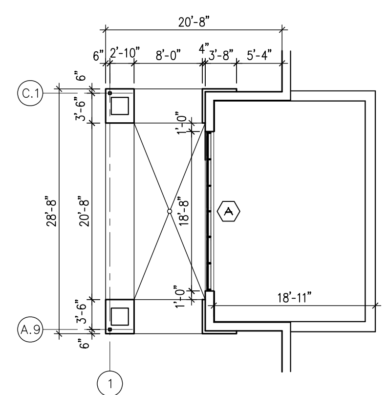
TOWER FLOOR PLAN 2 A1 3/32" = 1'-0"
